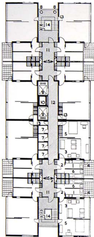
fig 140: Great Arthur House, typical floor plan
