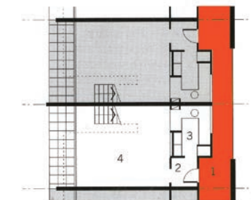
fig 143: Maisonette, lower floor fig 144: (left) typical section through Basterfield House
