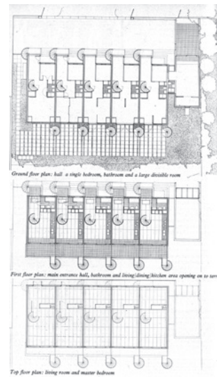
fig 175: Plans of the three floors fig 176: axonometry of the building pposite page, top left to bottom: fig 177: Entrance facade fig 178: Interior view fig 179: Sections through one unit fig 180: Bedrooms are combinable fig 181: Every corner is defined
