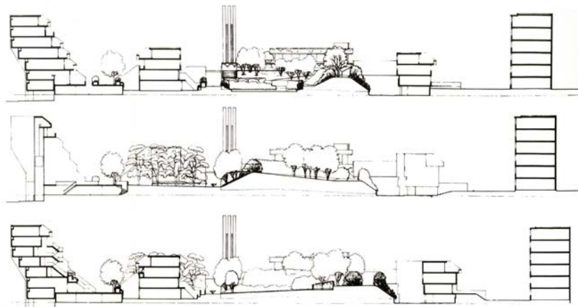
fig 199: Three main sections (north - south)
