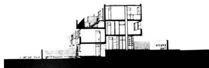
fig 209: Section through garden block
