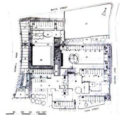
fig 133: Overview plan
