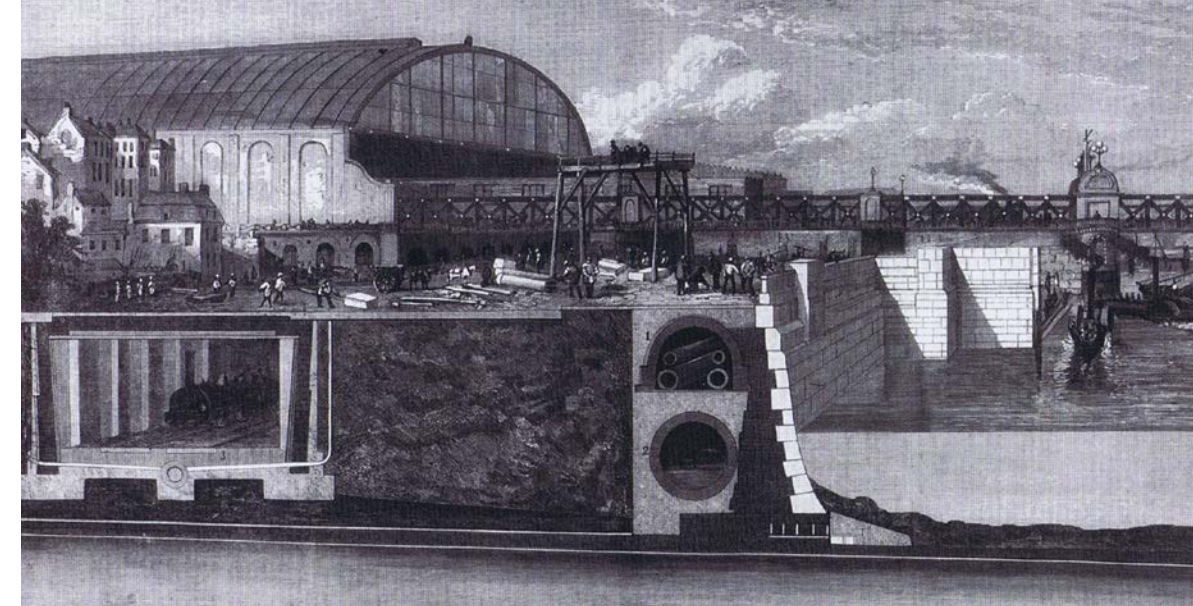
fig 44: A Cross-section through the Victorian Embankment
