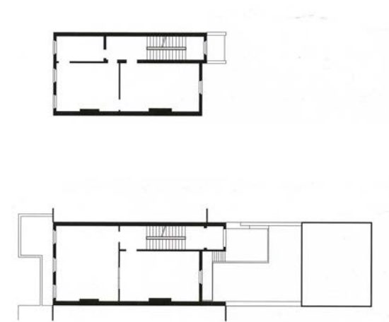
fig 99: first and second floor of house with mews
