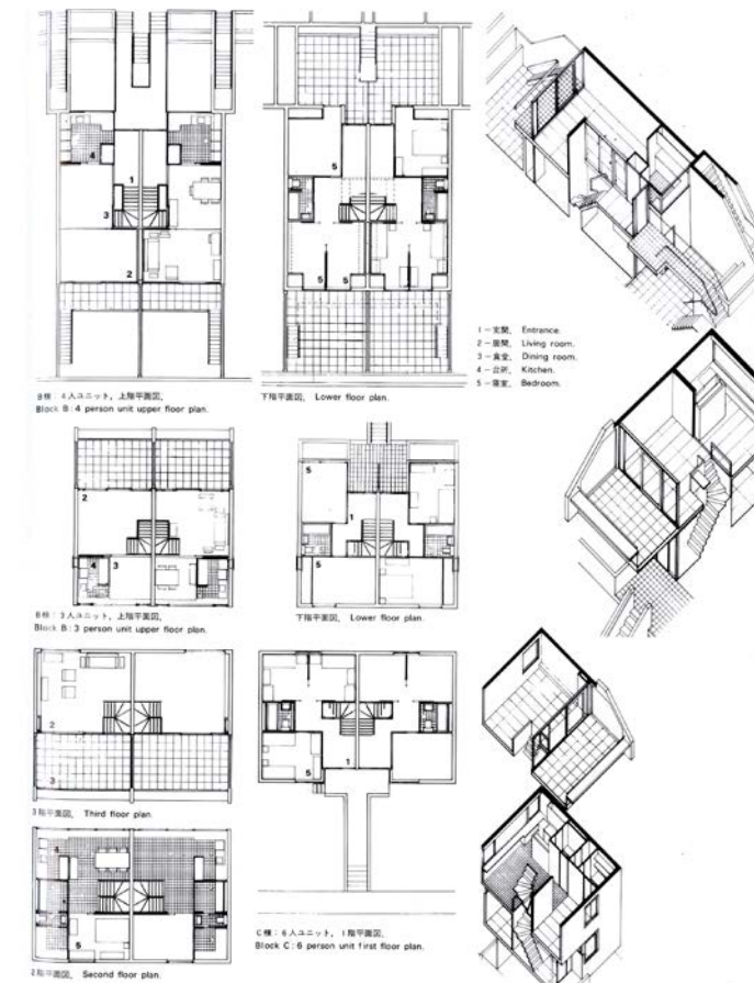
fig 196: (bottom) Plans and axonometric views of the different flat types
