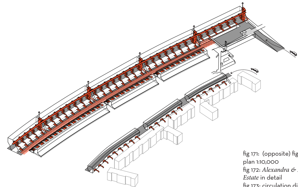
fig 173: circulation diagram
