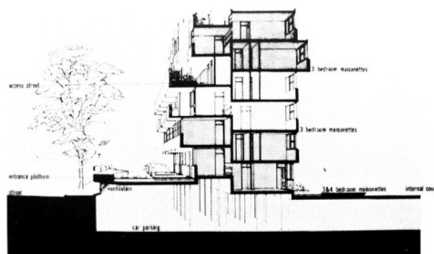
fig 207: Section through southern block along Tachbrook St
